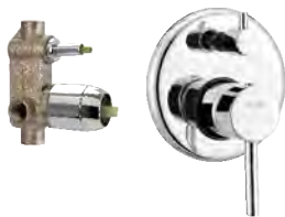
Turn type single lever concealed diverter system consisting of Exposed part (lever, tip ton knob, flange) and Concealed part (40 mm cartridge with button assembly, cartridge sleeve)
