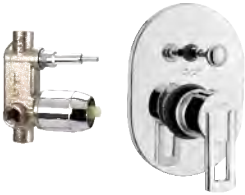
Single lever concealed diverter system consisting of Exposed part (lever, tip ton knob, flange) and Concealed part (40 mm cartridge with button assembly, cartridge sleeve)
