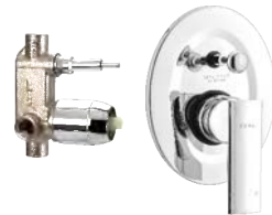
Single lever concealed diverter system consisting of Exposed part (lever, tip ton knob, flange) and Concealed part (40 mm cartridge with button assembly, cartridge sleeve) Exposed part F1003701 ₹ 2005 Concealed part F4010101 ₹ 3445 Set ₹ 5450
