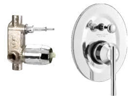
Single lever concealed diverter system consisting of Exposed part (lever, tip ton knob, flange) and Concealed part (40 mm cartridge with button assembly, cartridge sleeve) Exposed part F2003701 ₹ 1775 Concealed part F4010101 ₹ 3445 Set ₹ 5220
