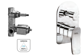
Turn type single lever concealed diverter system consisting of Exposed part (lever, turn type knob, 2 mm thick sheet metal wall flange) and Concealed part (35 mm cartridge with button assembly, cartridge sleeve) Exposed part F1012702 ₹ 2590 Concealed part F4010106 ₹ 4125 Set ₹ 6715
