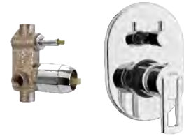
Turn type single lever concealed diverter system consisting of Exposed part (lever, turn type knob, flange) and Concealed part (40 mm cartridge with button assembly, cartridge sleeve)
