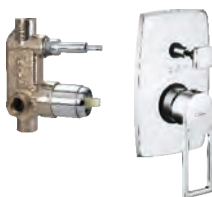
Single lever concealed diverter system consisting of Exposed part (lever, tip ton knob, flange) and Concealed part (35 mm cartridge with button assembly, cartridge sleeve) Exposed part F1099701 ₹ 1985 Concealed Part F4010103 ₹ 3020 Set ₹ 5005
