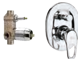
Turn type single lever concealed diverter system consisting of Exposed part (lever, turn type knob, flange) and Concealed part (40 mm cartridge with button assembly, cartridge sleeve)
