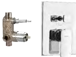
Single lever concealed diverter system consisting of Exposed part (lever, tip ton knob, flange) and Concealed part (35 mm cartridge with button assembly, cartridge sleeve) Exposed part F1005701 ₹ 2345 Concealed part F4010103 ₹ 3020 Set ₹ 5365
