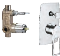
Single lever concealed diverter system consisting of Exposed part (lever, tip ton knob, 2 mm sheet flange) and Concealed part (35 mm cartridge with button assembly, cartridge sleeve) Exposed part F1099702 ₹ 1985 Concealed Part F4010103 ₹ 3020 Set ₹ 5005
