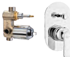
High flow single lever concealed diverter system consisting of Exposed part (lever, tip ton knob, flange) and Concealed part (45 mm cartridge with button assembly, cartridge sleeve) Exposed part F1018721 ₹ 2525 Concealed Part F4030101 ₹ 4115 Set ₹ 6640
