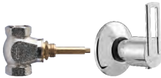
Flush cock consisting of exposed part (lever, cartridge sleeve, flange) and concealed part Exposed part F1007751 ₹ 520 Concealed part F4060102 ₹ 2300 Set ₹ 2820 Light weight concealed part F4060101 ₹ 1725 concealed part F4060103 ₹ 1510 concealed part F4060104 ₹ 1890
