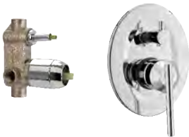
Turn type single lever concealed diverter system consisting of Exposed part (lever, tip ton knob, flange) and Concealed part (40 mm cartridge with button assembly, cartridge sleeve)
