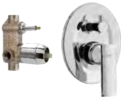
Turn type single lever concealed diverter system consisting of Exposed part (lever, turn type knob, flange) and Concealed part (40 mm cartridge with button assembly, cartridge sleeve) Exposed part F1003703 ₹ 2005 Concealed part F4010105 ₹ 3520 Set ₹ 5525
